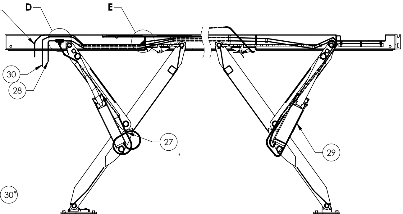
SECTION C-C SCALE 1 : 25
